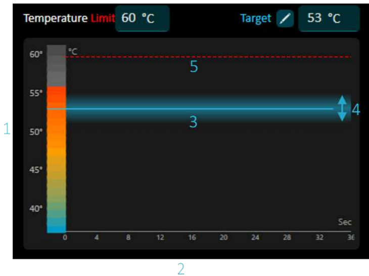
Figure 9-6: Temperature Graph
