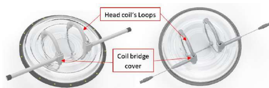
Figure 1-18: Examples of Tc MRgFUS Head Coil
