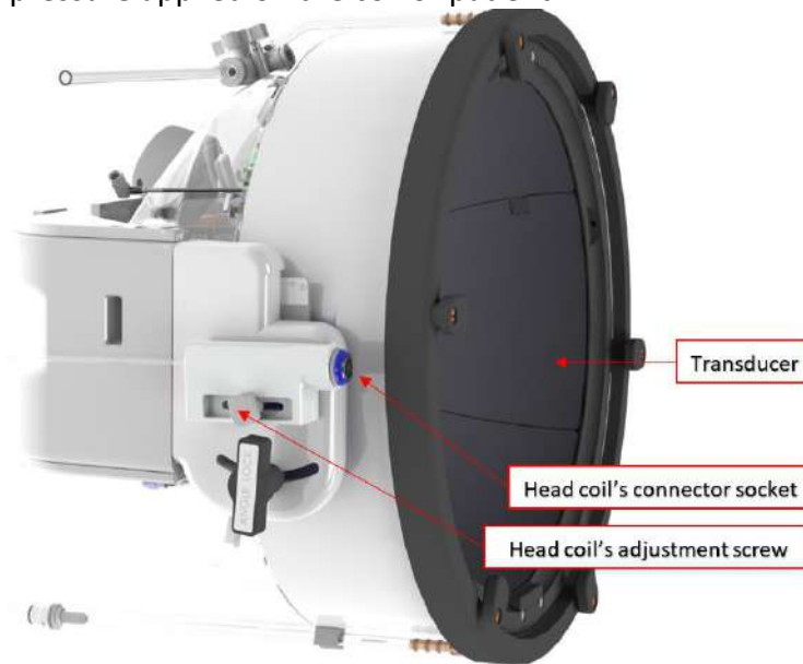
Figure 1-20: Head Coil connector socket.
