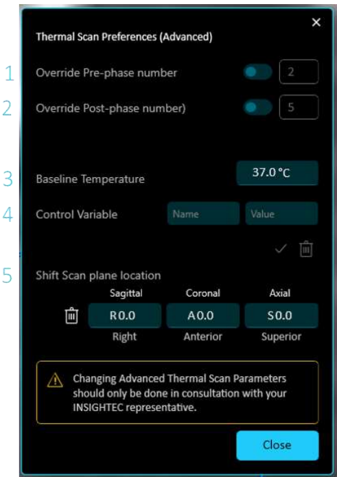
Figure 9-15: Advanced Thermal Scan Preferences Menu
