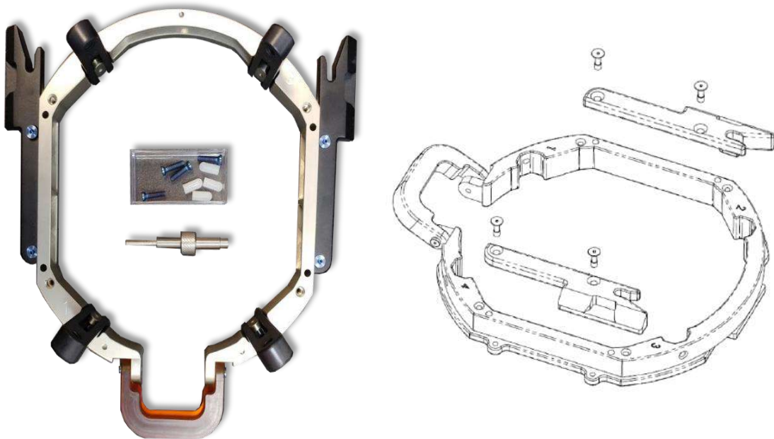
Figure A - 2: Connecting Side Holders to the Headframe (for illustration purposes only)
