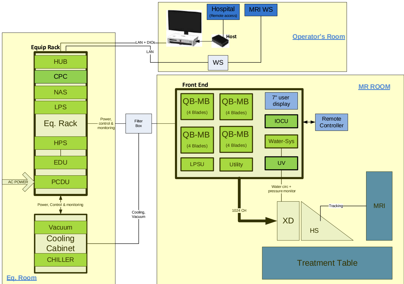
Figure 1-1: Schematic Representing Layout of System Components In-Site
