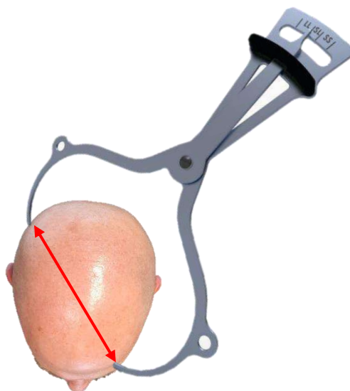
Figure 13-5 - Exablate Caliper for Head diagonal measurement and combination estimation
