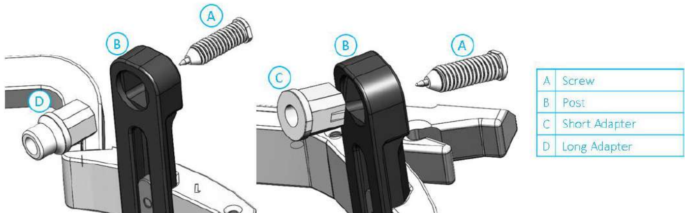
Figure A - 7: Internal Adapter insertion to posts
