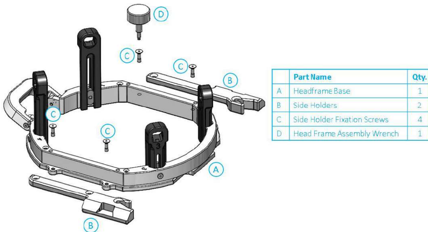
Figure 1-15: Connecting Side Holders to the Headframe (for illustration purposes only)
